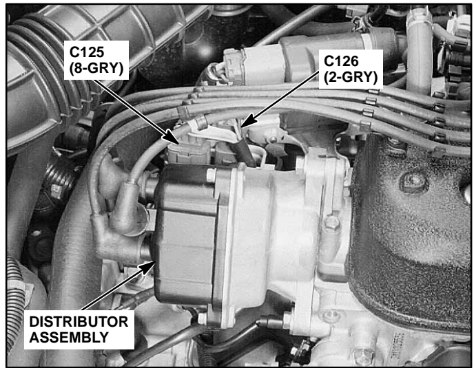
11. Right Side of 2.3L Engine (2.2L DOHC Similar)
