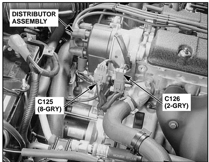
12. Right Side of 2.3L Engine (2.2L Similar)
