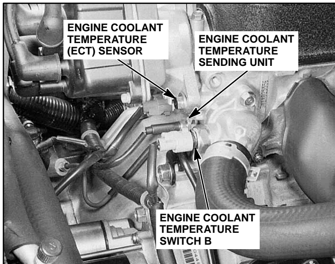
9. Right Side of 2.2L SOHC Engine (Others Similar)
