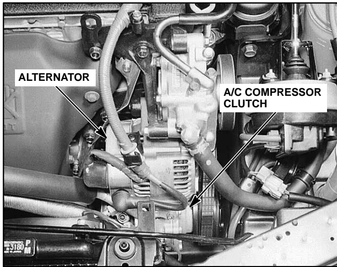
8. Left Front of Engine
