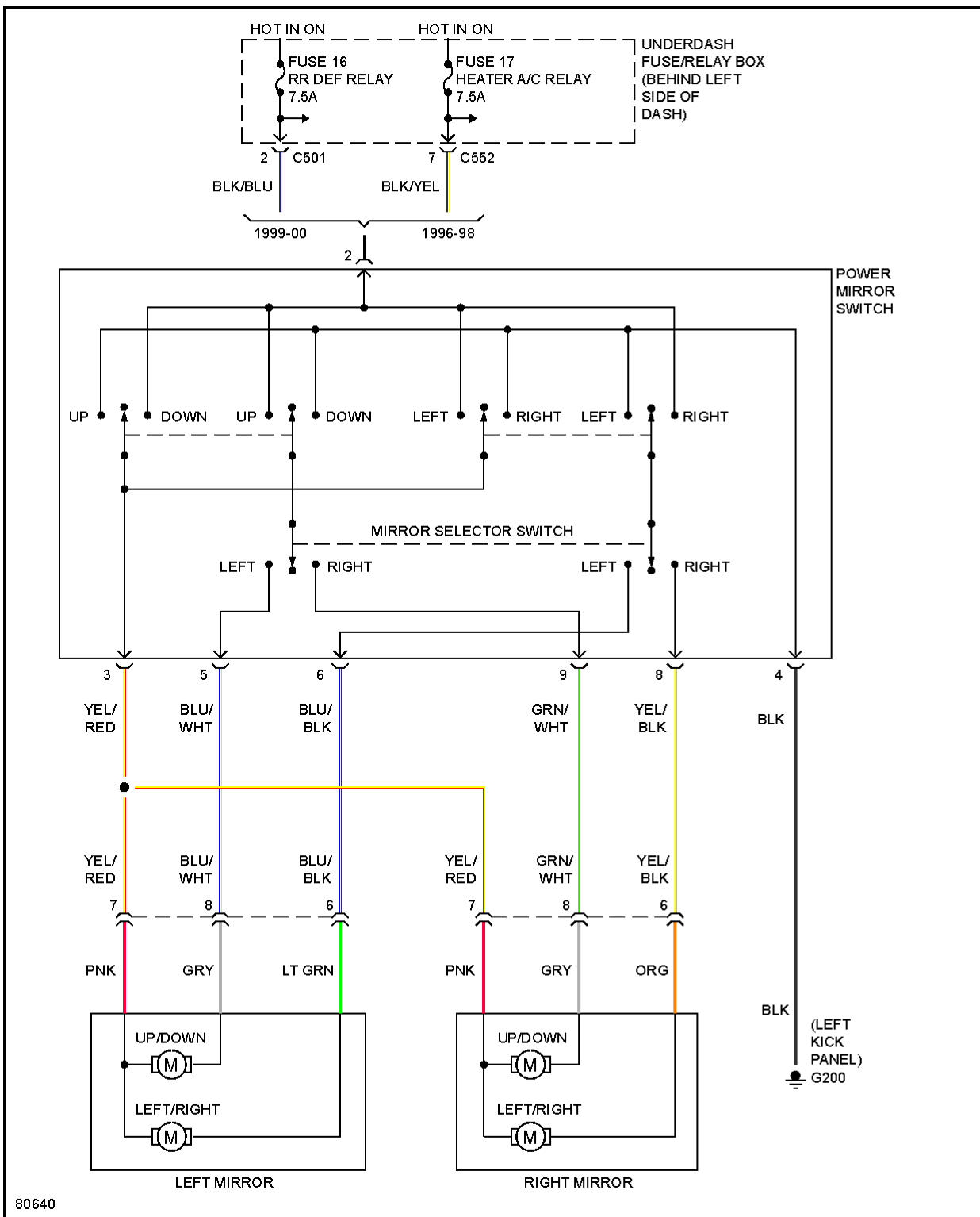
Fig. 42: Power Mirror Circuit
