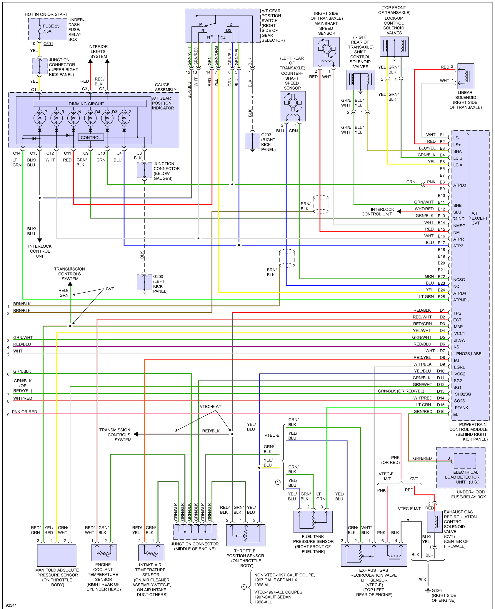
Fig 12: Wiring Diagram (Civic 1.6L - 3 Of 3)
