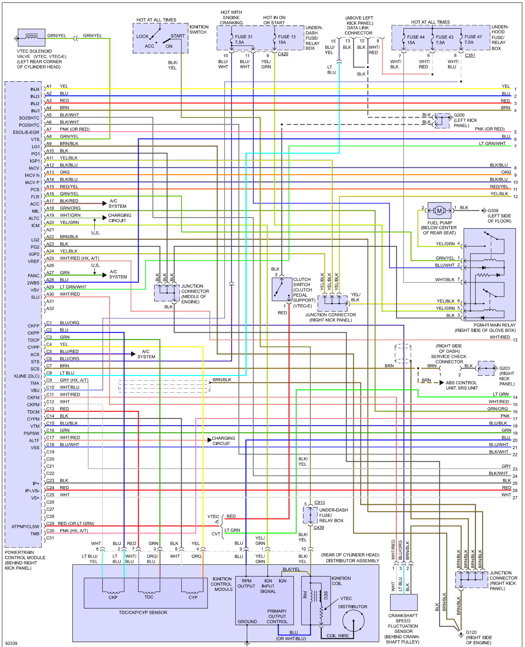
Fig 10: Wiring Diagram (Civic 1.6L - 1 Of 3)
