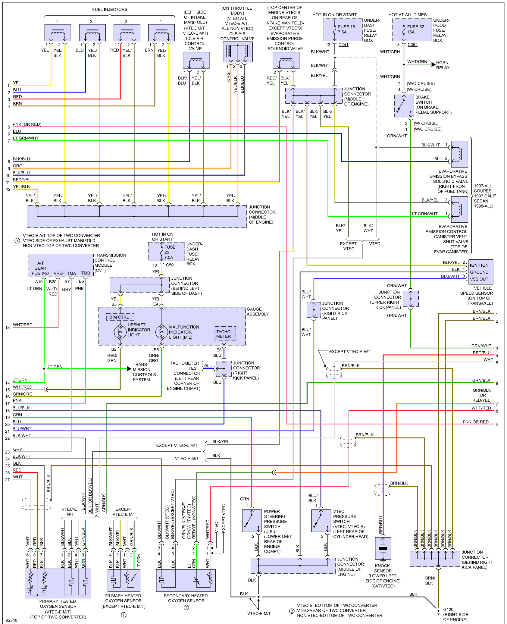
Fig 11: Wiring Diagram (Civic 1.6L - 2 Of 3)
