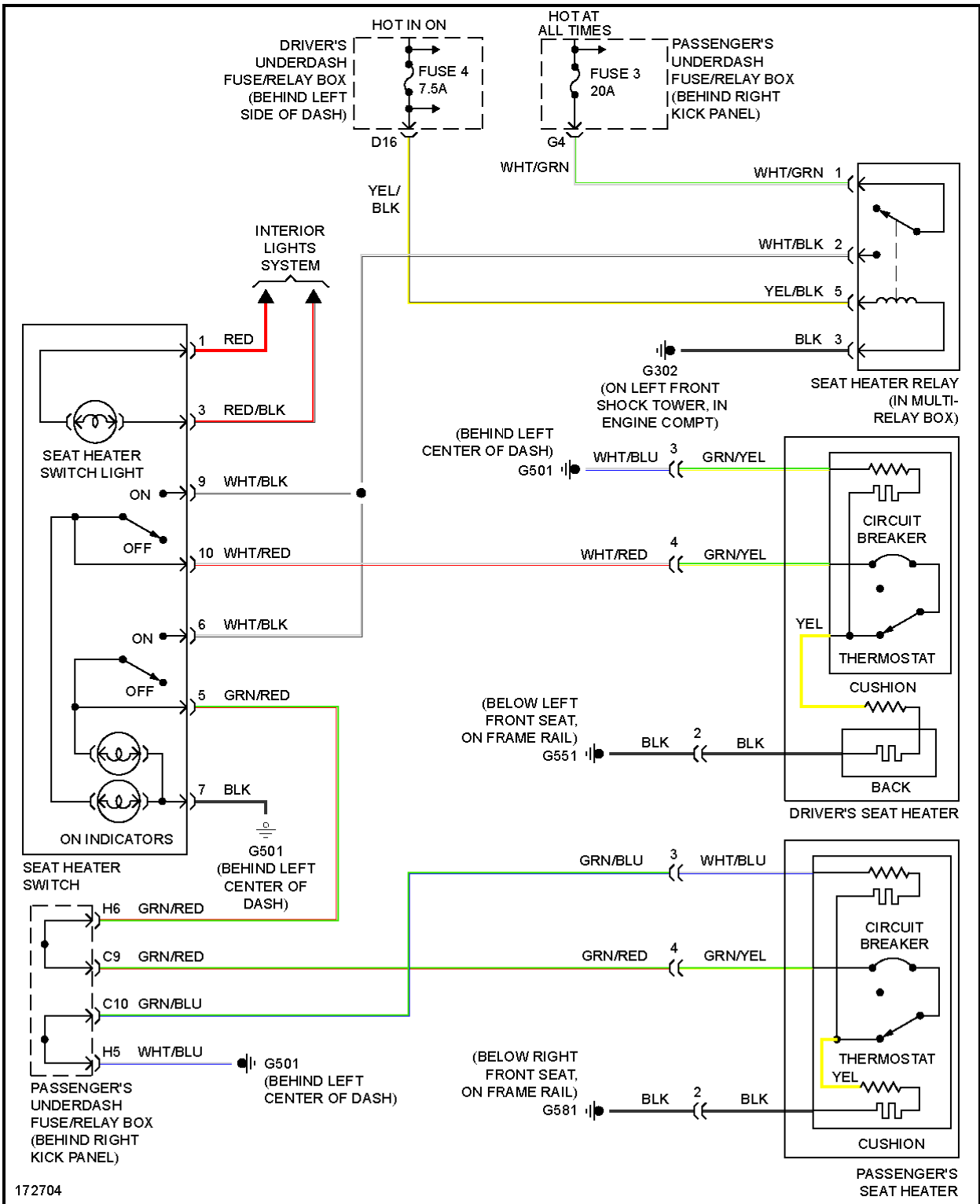
Fig. 65: Heated Seats Circuit, M/T
