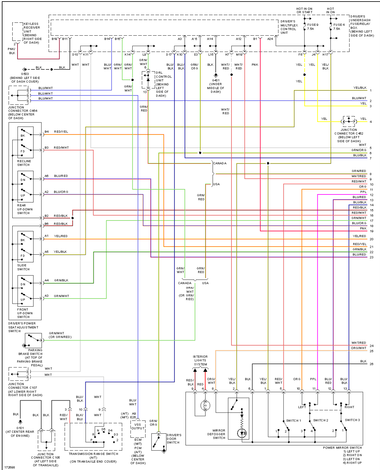
Fig. 52: Memory Systems Circuit (1 of 3)
