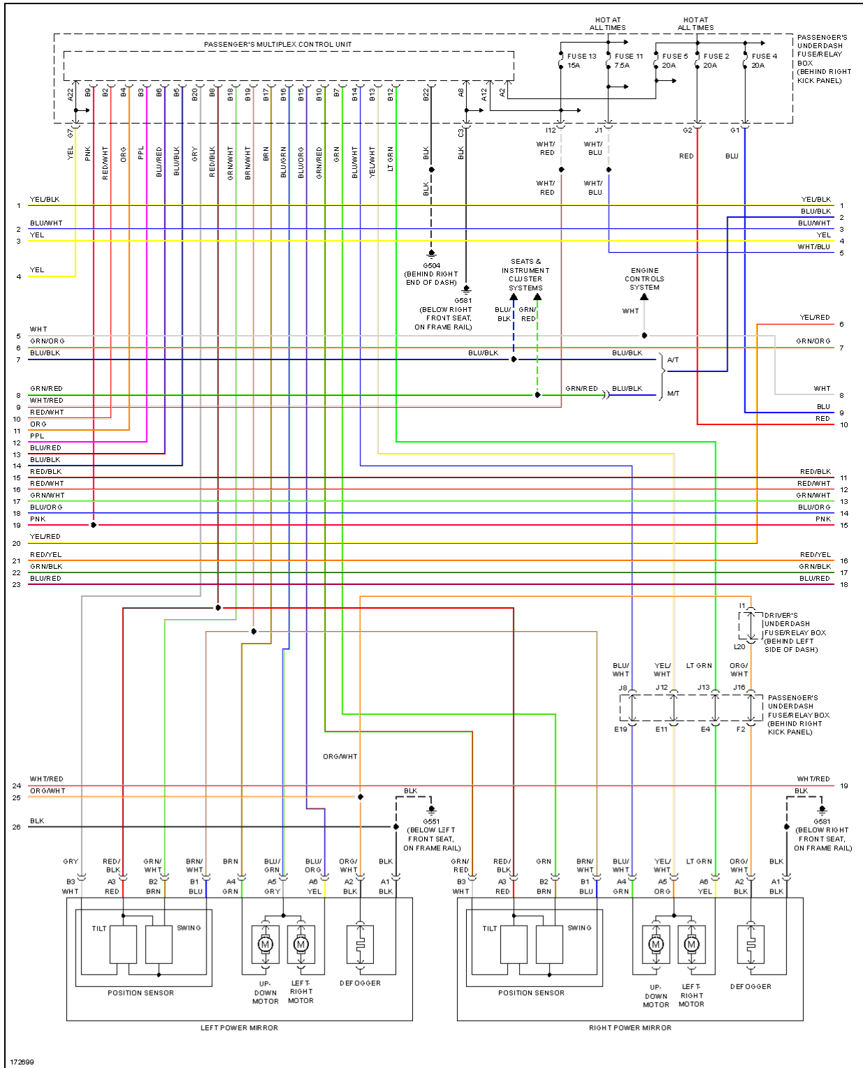
Fig. 53: Memory Systems Circuit (2 of 3)
