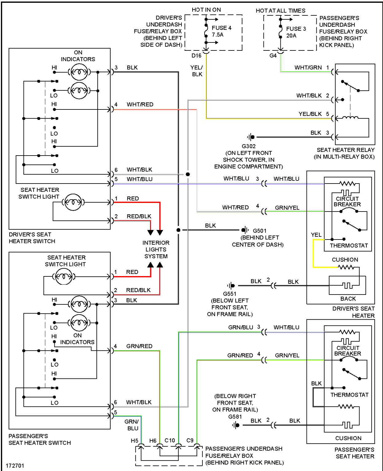
Fig. 64: Heated Seats Circuit, A/T
