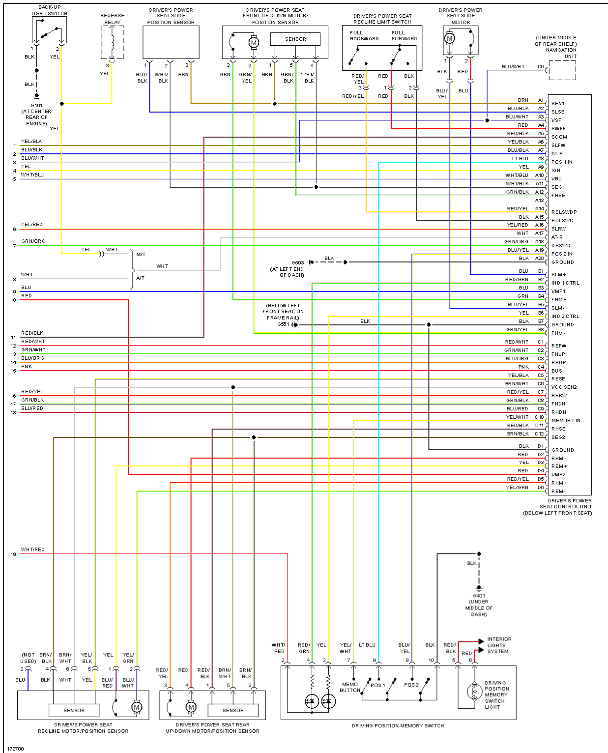
Fig. 54: Memory Systems Circuit (3 of 3)
