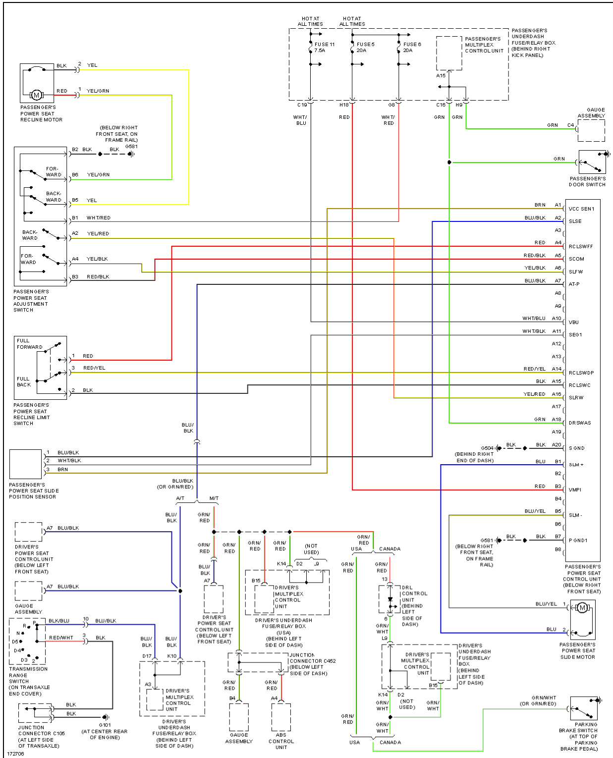
Fig. 66: Passenger Power Seat Circuit
