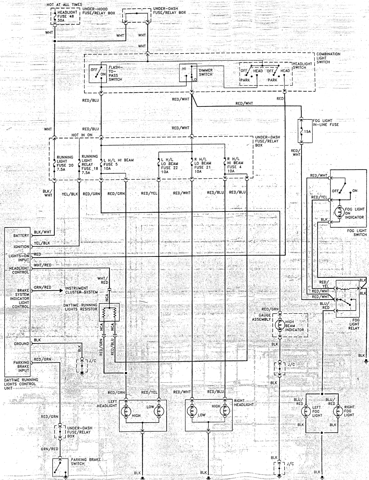
Headlight and fog light system - Civic
