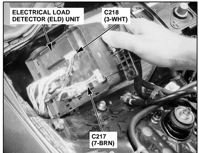
24. Rear of Under-hood Fuse/Relay Box
