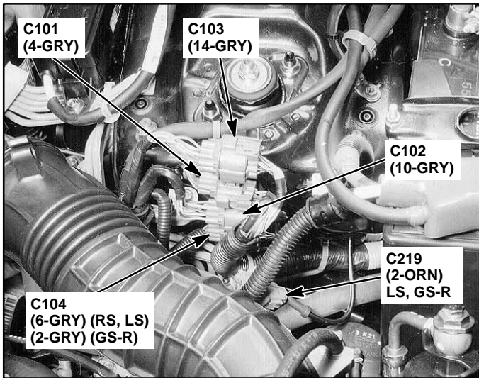
21. Right Rear Corner of Engine Compartment
