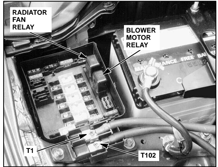
23. Rear of Under-hood Fuse/Relay Box
