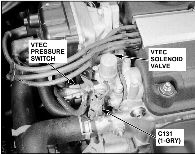
20. Right Side of Engine Compartment
