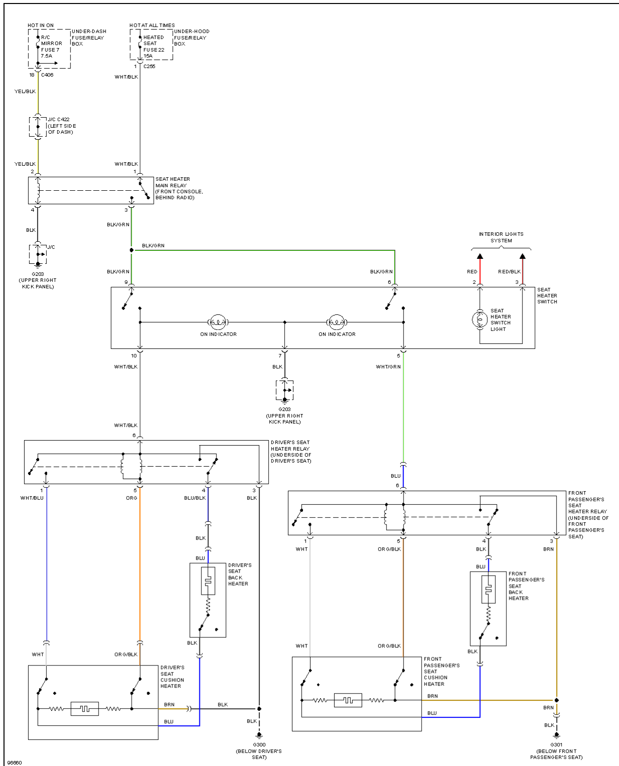
Fig. 10: Heated Seats System Wiring Diagram
