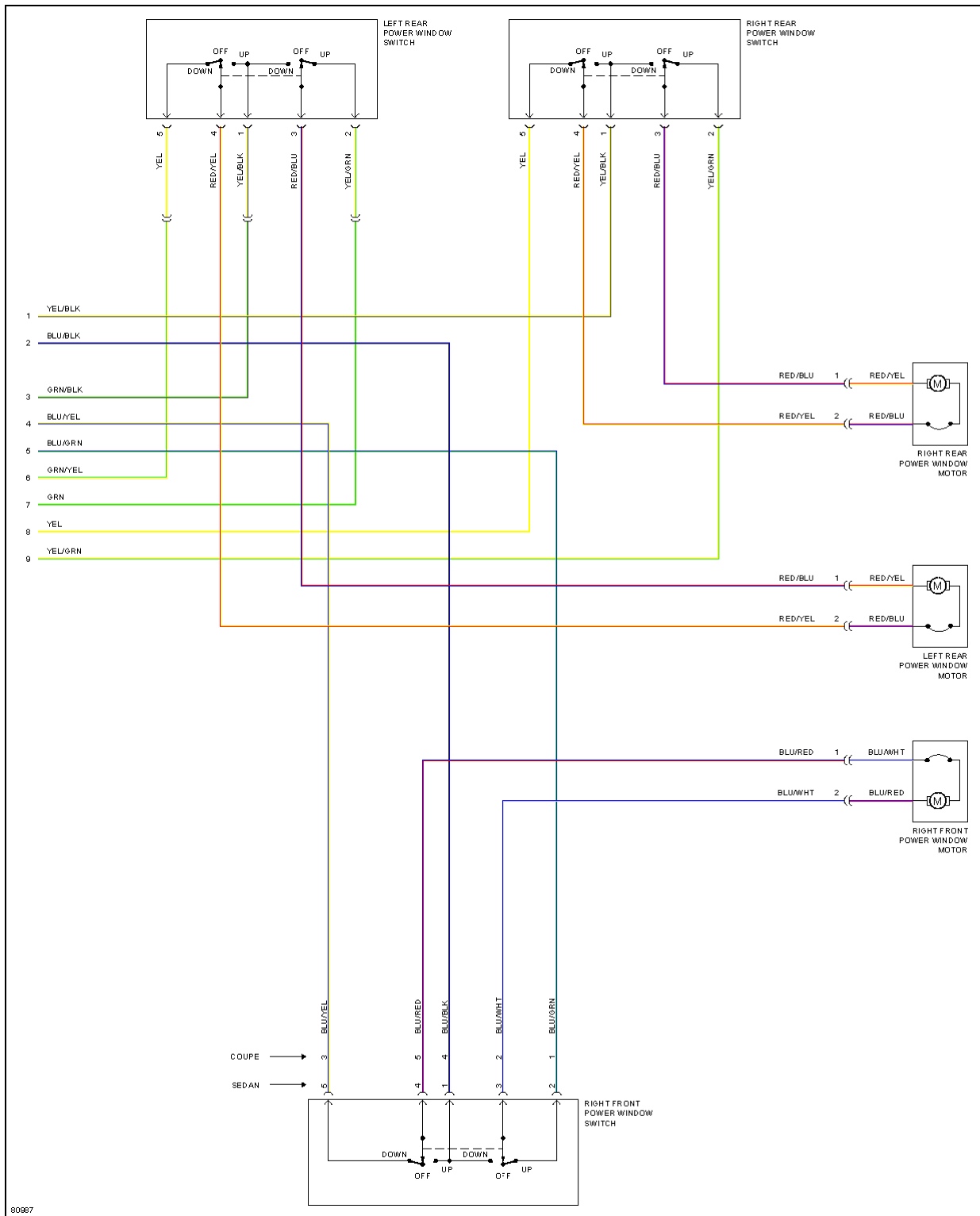
Fig. 40: Power Window Circuit (2 of 2)
