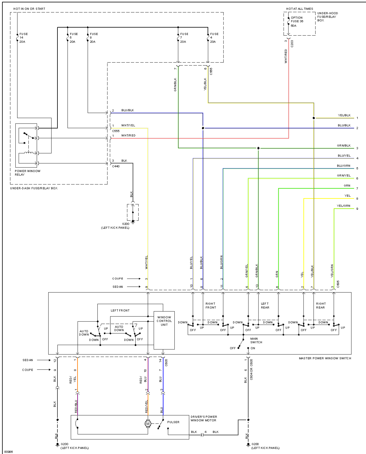
Fig. 39: Power Window Circuit (1 of 2)
